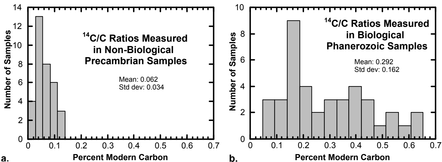
Figure 2. Distribution of ^{14}\text{C} values for (a) non-biogenic samples and (b) biogenic samples from Table 1. Given their position in the geological record, all these samples should contain no detectable ^{14}\text{C} according to the standard geological time scale.
