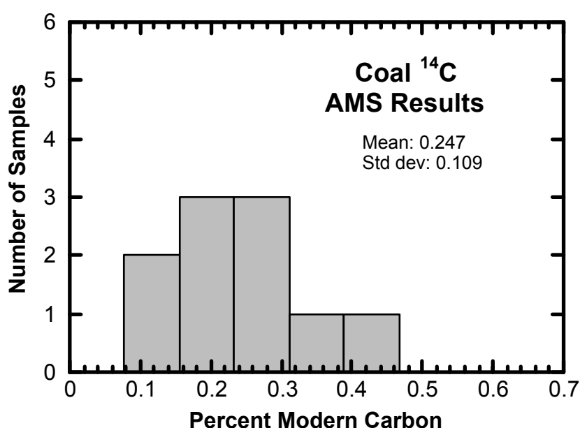
Figure 3. Histogram representation of AMS ^{14}\text{C} analysis of ten coal samples undertaken by RATE ^{14}\text{C} research project.
